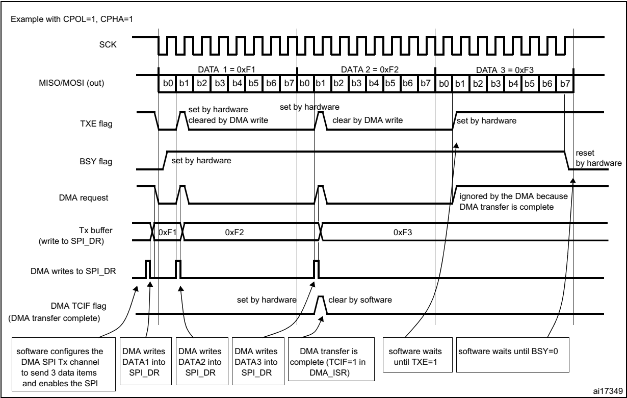
Figure 246. Transmission using DMA
