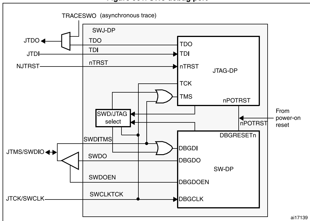
Figure 361. SWJ debug port
