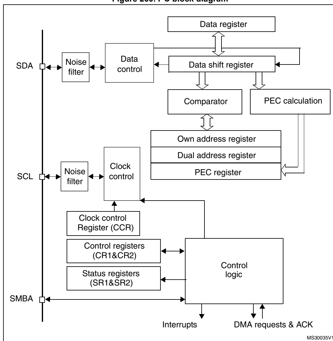
Figure 269. I 2 C block diagram
