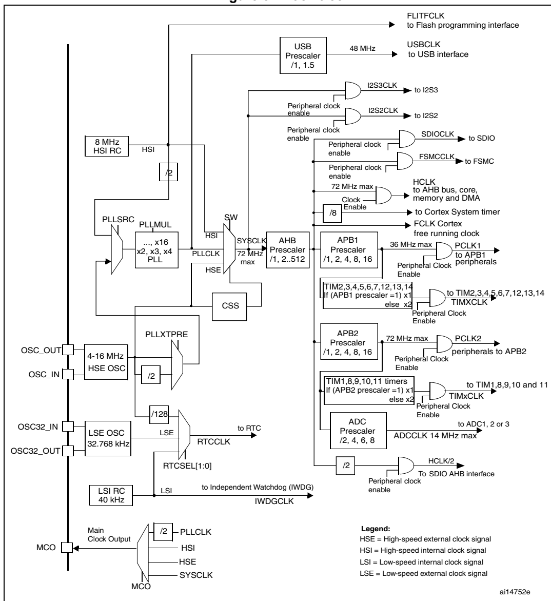
Figure 8. Clock tree
